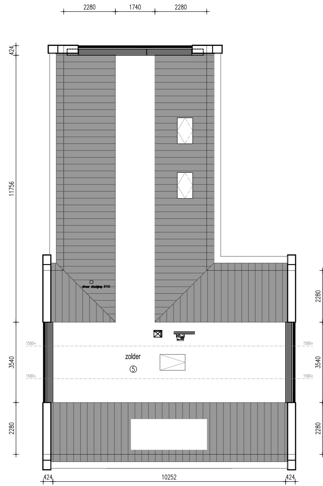
ZOLDER
